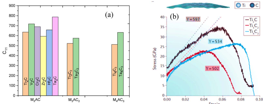
Fig. 17 (a) Calculated elastic constant values for various MXenes. (b) MXene stress–strain curves for \text{Ti}_2\text{C} , \text{Ti}_3\text{C}_2 , \text{Ti}_4\text{C}_3 . Reproduced from ref. 15 with permission from Springer Nature, copyright 2017.
