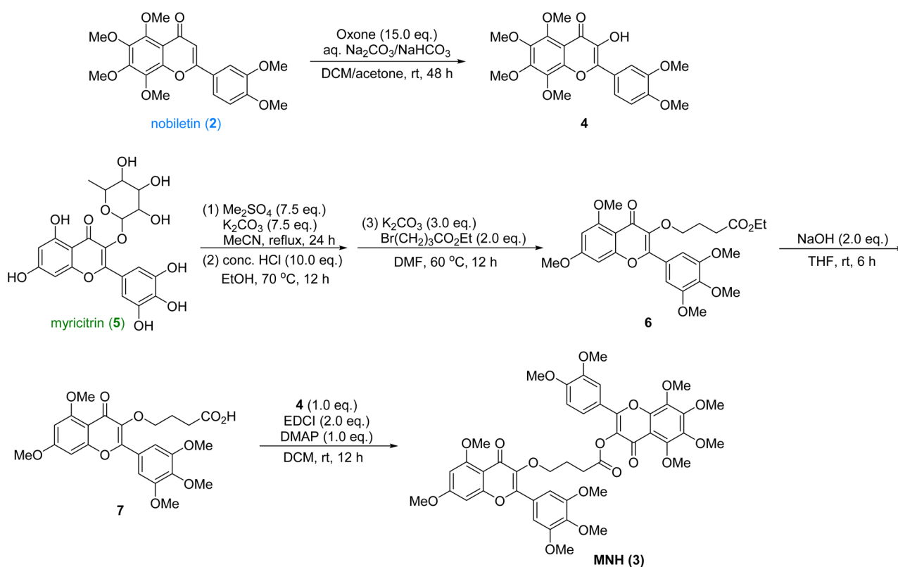
Scheme 1 Synthesis of MNH.
