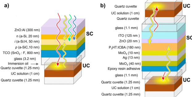
Fig. 7 Illustration of the device structure of TTA-UC solution integrated thin film solar cell, (a) a-Si:H p-i-n solar cell and (b) P 3 HT:ICBA organic photovoltaic solar cell (OPV). The TTA-UC solution on both sides of OPV indicates that it can be placed either below the ITO cathode or below the Ag anode. Transmitted red light is injected back into the solar cell in the form of upconverted to yellow light.
