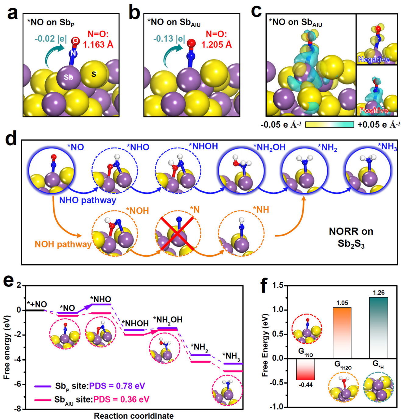
Fig. 3 (a and b) Atomic structures of absorbed NO on (a) the \text{Sb}_\text{P} site and (b) the \text{Sb}_\text{AIU} site of \text{Sb}_2\text{S}_3 . (c) Charge density difference of *NO on the \text{Sb}_\text{AIU} site (yellow: accumulation; cyan: depletion). (d) Schematic of two NORR pathways (NHO and NOH) on \text{Sb}_2\text{S}_3 . (e) Free energy profiles of the NORR process (NHO pathway) on \text{Sb}_\text{P} and \text{Sb}_\text{AIU} . (f) Binding free energies of *H 2 O, *H and *NO on \text{Sb}_\text{AIU} .
