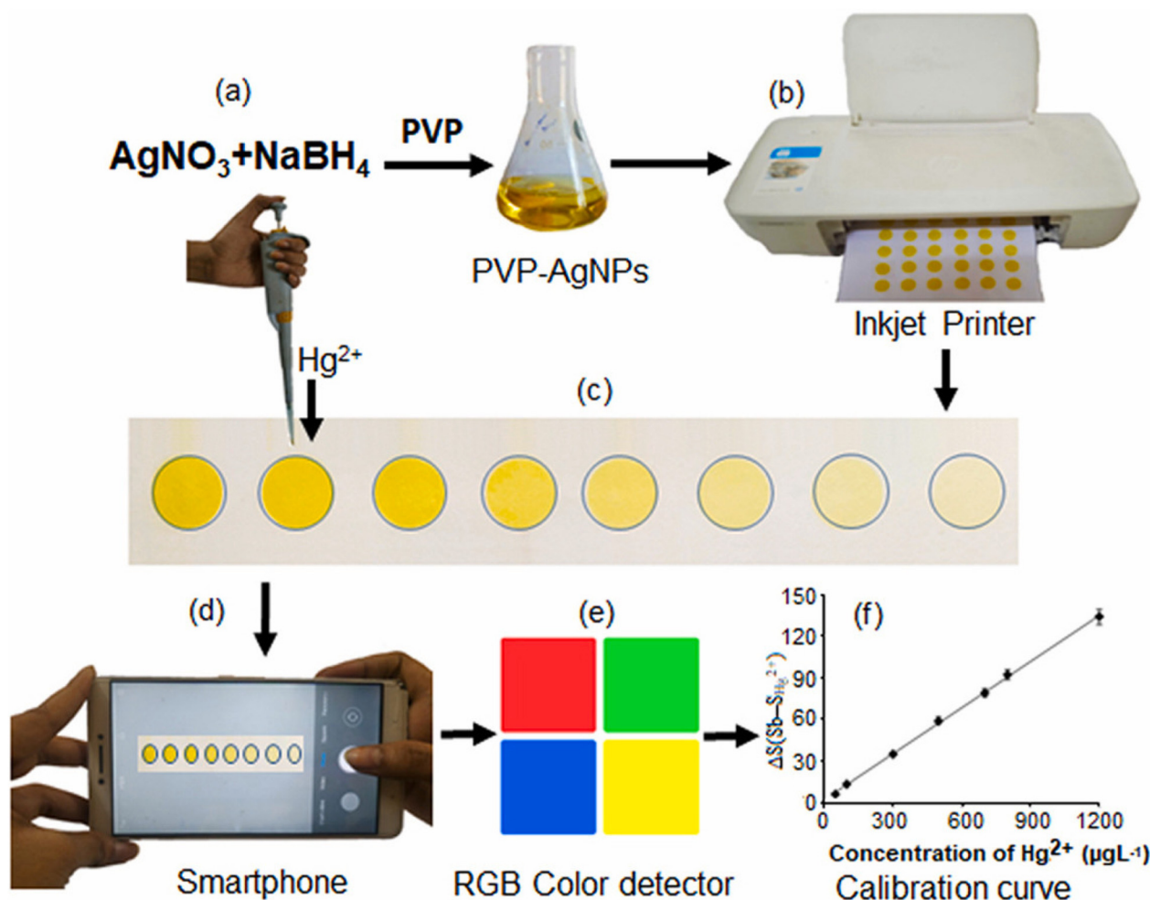
Fig. 6 Systematic representation of the development of an AgNPs-PVP-based portable colorimetric sensor. (a) Synthesis of AgNPs-PVP. (b) Printing of AgNPs in filter paper in an AgNP sensing probe. (c) Pipetting \text{Hg}^{2+} in an AgNP sensing probe. (d) Image captured using a smartphone. (e) RGB value analyzed using ImageJ software. (f) The result as a calibration curve [this figure has been reproduced from ref. 60 with permission from Elsevier Sciences, copyright 2021].
