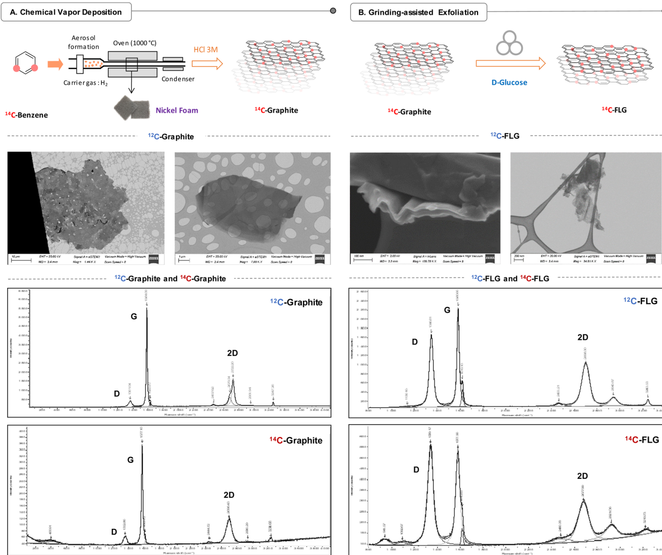
Fig. 2 (A) Synthesis and characterization of 14 C-graphite. Upper panel: schematic representation of the CVD preparation of 14 C-graphite from 14 C-benzene. Middle panel: morphological characterization of 12 C-graphite by STEM. Scale: 10 μm (left) and 1 μm (right). Lower panel: Raman spectra of 12 C-graphite (up) and 14 C-graphite (down). (B) Synthesis and characterization of 14 C-FLG. Upper panel: schematic representation of the grinding-assisted exfoliation of 14 C-graphite to provide 14 C-FLG. Middle panel: morphological characterization of 12 C-FLG by STEM. Scale: 100 nm (left) and 200 nm (right). Lower panel: Raman spectra of 12 C-FLG (up) and 14 C-FLG (down).
