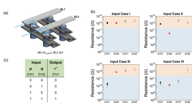
Fig. 5 Experimental demonstration of the AND logic gate between D_{11t} and D_{12t} memristors in the BLC. (a) The bias configuration in the schematic diagram of the vertical CBA, where V_{a,\text{AND}} = +9 V. (b) The results of the AND logic operation in D_{11t} for each input case. A resistance lower than 250 G \Omega is encoded to the "1" state and (c) its truth table of the logic gate.
