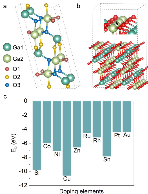
Fig. 1 (a) Schematic representation of the unit cell of \beta\text{-Ga}_2\text{O}_3 . (b) Schematic representation of (100) \beta\text{-Ga}_2\text{O}_3 surface. Colour code: Ga1, dark green; Ga2, light green; O, red. The star indicates this Ga will be substituted by other elements. (c) The binding energy ( E_b ) of various elements on the (100) \beta\text{-Ga}_2\text{O}_3 surface.
