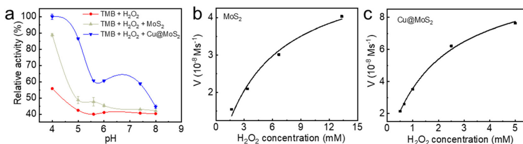
Fig. 5 (a) Relative catalytic activity of the \text{MoS}_2 and \text{Cu@MoS}_2 as peroxidase mimics under different pH values at 37 °C tested by UV-vis absorption of oxTMB. The velocity of the reaction between \cdot\text{OH} and the various concentrations of \text{H}_2\text{O}_2 in the presence of (b) \text{MoS}_2 and (c) \text{Cu@MoS}_2 . The successful Cu loading on the \text{MoS}_2 surface was well in agreement with the DFT calculations.
