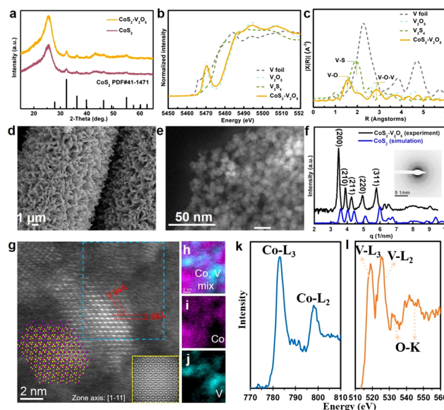
Fig. 2 Structural analysis of \text{CoS}_2\text{-V}_2\text{O}_5 . (a) XRD patterns of \text{CoS}_2 and \text{CoS}_2\text{-V}_2\text{O}_5 , (b) V K-edge XANES of \text{CoS}_2\text{-V}_2\text{O}_5 , V foil, \text{V}_2\text{O}_5 and \text{V}_2\text{S}_4 , (c) V K-edge EXAFS of \text{CoS}_2\text{-V}_2\text{O}_5 , V foil, \text{V}_2\text{O}_5 and \text{V}_2\text{S}_4 , (d) SEM image of \text{CoS}_2\text{-V}_2\text{O}_5 nanoarrays loaded on CC, (e) HAADF-STEM image of \text{CoS}_2\text{-V}_2\text{O}_5 particles, (f) radial intensity profile of \text{CoS}_2\text{-V}_2\text{O}_5 (black line) and the simulated radial intensity profile of \text{CoS}_2 (blue line), inset shows the SAED of \text{CoS}_2\text{-V}_2\text{O}_5 , (g) atomic HAADF-STEM image of \text{CoS}_2\text{-V}_2\text{O}_5 along with the zone axis [1–11] direction (inset shows the atomic model of \text{CoS}_2 ), (h) cobalt and vanadium colormix, (i) cobalt mapping, (j) vanadium mapping, EELS spectra of k cobalt L edge, (l) oxygen K edge, and vanadium L edge acquired from the blue rectangular region in (g).
