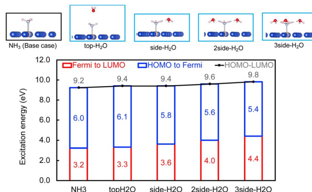
Fig. 1 The effect of \text{H}_2\text{O} molecules on the interfacial charge and energy transfer. Top panel: Optimized configurations of \text{NH}_3 on \text{RuCu}_{83} with and without \text{H}_2\text{O} . Bottom: the excitation energy required to excite an electron from the HOMO of \text{NH}_3 to the Fermi level (blue), from the Fermi level to the LUMO of \text{NH}_3 (red), and from the HOMO to the LUMO by adding the two excitation energy values (black).
