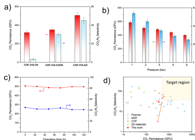
Fig. 4 Separation performances of membranes. (a) \text{CO}_2/\text{N}_2 (20/80 vol%) mixed-gas separation performances of COF membranes at 100% relative humidity, 298 K and 2 bar. (b) The performance of COF-316-AO under feed gas pressure of 1–5 bar. (c) Long-term test of COF-316-AO membrane tested at 2 bar and 100% relative humidity. (d) Comparison of the \text{CO}_2/\text{N}_2 separation performances of the membranes and representative membranes in the literature. The light-yellow region is the target area for post-combustion capture of \text{CO}_2 . 29,30 The data were obtained from the previous literature listed in Table S1 (ESI † ).
