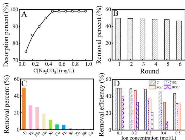
Fig. 6 Effect of Na 2 CO 3 concentration on the desorption of U(vi) from K 2 FeO 4 @PAO (A); recycling of K 2 FeO 4 @PAO in the extraction of U(vi) from solution (B); comparison of K 2 FeO 4 @PAO adsorption performance for 10 mg L -1 U(vi) and heavy metal ions (C); U(vi) removal efficiency for K 2 FeO 4 @PAO with the coexistence of different anions (D). I = 0.1 \text{ mol L}^{-1} NaCl, T = 298 \pm 1 \text{ K} , contact time: 24 h. C[\text{U(vi)}]_{\text{initial}} = 10.0 \text{ mg L}^{-1} , m = 0.02 \text{ g} , V = 50 \text{ mL} , \text{pH} = 8.2 \pm 0.1 .
