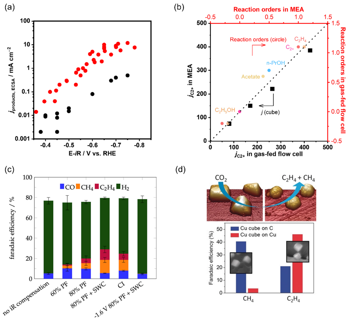
Fig. 10 (a) Comparison of \text{C}_2\text{H}_4 partial current densities normalized to ECSA of CO electroreduction on Cu in a gas-fed flow cell and H-type cell. The data is adapted from ref. 145, 149, 150, 199, 200 (b) Comparison of as-obtained kinetic results ( j_{\text{C}_2\text{H}_4} and reaction orders) in a gas-fed flow cell and MEA under the same reaction conditions during CO electroreduction over Cu. The data is adapted from ref. 145. (c) Product distributions with different iR compensations at -1.7 \text{ V vs. Ag/AgCl} in CO 2 saturated 0.1 M KHCO 3 . Reproduced with permission. 204 Copyright 2022, American Chemical Society. (d) Dynamic changes in the structure and catalytic selectivity of Cu nanocubes in CO 2 electroreduction. Reproduced with permission. 205 Copyright 2018, Wiley-VCH.
