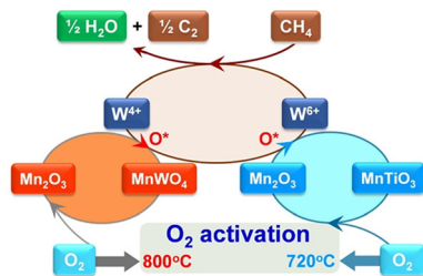
Fig. 6 Proposed catalytic cycle for OCM reaction mediated by the redox cycle \text{Mn}^{2+} \leftrightarrow \text{Mn}^{3+} over \text{Mn-Na}_2\text{WO}_4/\text{Ti-MWW} . Reprinted from ref. 36 with permission from The American Association for the Advancement of Science, copyright 2017.
