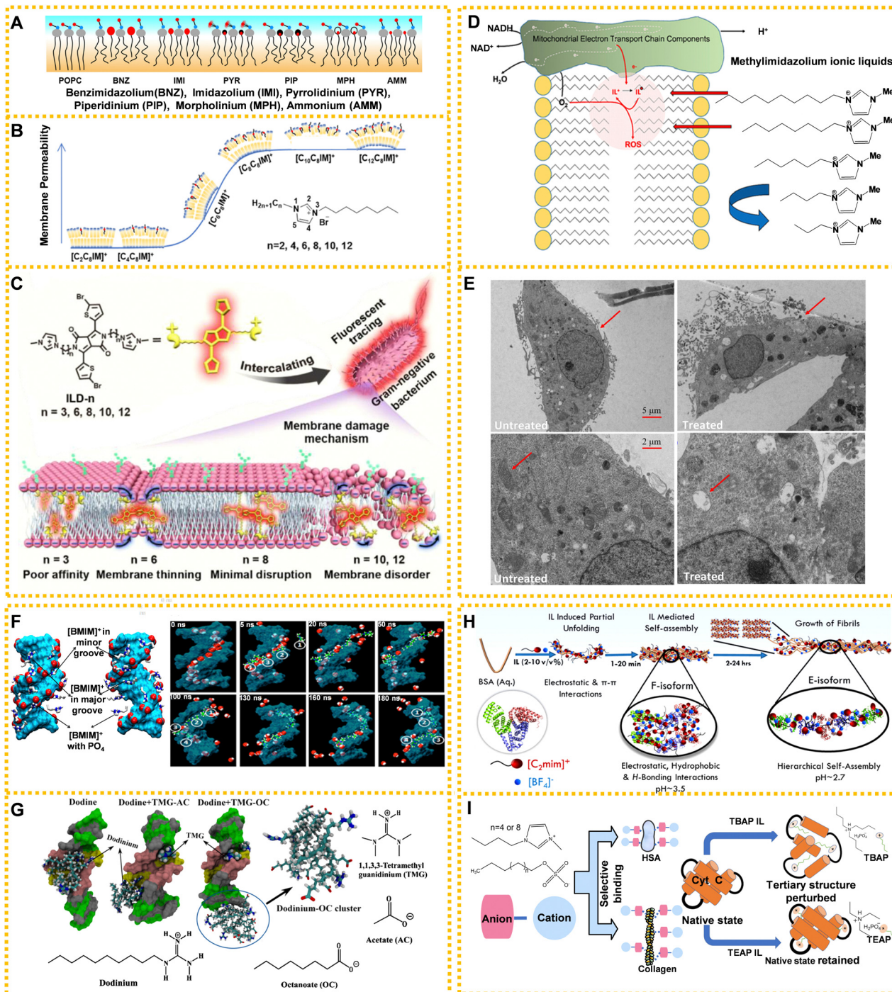
Fig. 5 Ions acting on living organisms: (A) schematic models of different ILs' head-group size, hydrophobicity, and charge delocalization impacting the structure of 2-oleoyl-1-pamitoyl- sn -glycero-3-phosphocholine (POPC) bilayer. Black wavy lines: alkyl chains in lipids and cations, grey filled circles: glycerol moieties in the lipid head-groups, blue and red filled circles connected with black lines: phosphocholine dipoles, and red circles: head-groups of cations intercalated in lipid molecules. Reproduced with permission from ref. 148. Copyright 2020 Elsevier. (B) The leakage kinetics of calcein dye from POPC and 2-oleoyl-1-pamitoyl- sn -glycero-3-phosphoglycerol (POPG) large unilamellar vesicles and the regular model of membrane permeability associated with ILs' cations. Reproduced with permission from ref. 149. Copyright 2021 American Chemical Society. (C) The membrane damage mechanism of ILs with different chain lengths on Gram-negative bacteria. Reproduced with permission from ref. 151. Copyright 2020 American Chemical Society. (D) Methylimidazolium ILs affecting the mitochondrial electron transport chain in mammalian cells. Reproduced with permission from ref. 152. Copyright 2020 Elsevier. (E) The effects of [C 10 MIM][Cl] on mitochondria of HeLa cells with the original TEM images (top) and zoomed TEM images (bottom). Reproduced with permission from ref. 141. Copyright 2021 Elsevier. (F) Distribution map of the IL interaction with DNA. Cyan: DNA, red: DNA phosphates, white: IL cations, and blue: ring nitrogen of IL cations. Reproduced with permission from ref. 153. Copyright 2012 American Chemical Society. (G) The mechanism for ILs' long hydrocarbon chains of anions preventing a fungicide from destroying structural DNA. Reproduced with permission from ref. 154. Copyright 2020 American Chemical Society. (H) The formation mechanism for bovine serum albumin (BSA) amyloid fiber in the presence of [EMIM][BF 4 ] (2–10 v/v%). Reproduced with permission from ref. 155. Copyright 2021 American Chemical Society. (I) The effect and relationship between the length of alkyl chain of anion (left) and cation (right) on proteins. Reproduced with permission from ref. 156 and 157. Copyright 2018 Royal Society of Chemistry and 2020 American Chemical Society.
