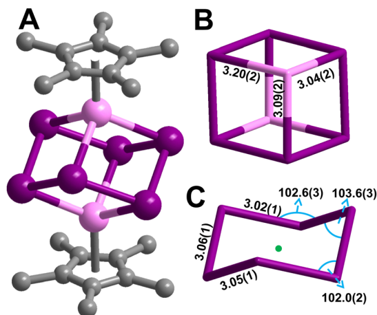
Fig. 1 (A) Structure of [K(THF) 4 ] 2 [Cp* 2 Y 2 Bi 6 ] ( 1 ). Pink, purple, and grey spheres represent Y, Bi, and C atoms, respectively. H atoms and both [K(THF) 4 ] + cations have been omitted for clarity. (B) Neutral {Y 2 Bi 6 } cube enlarged with Y–Bi distances labelled. (C) Bi 6 6− chair enlarged with distances and angles labelled. The green mark represents the inversion centre. All distances (Å) and angles (°) are rounded up for clarity and full values are in the main text.
