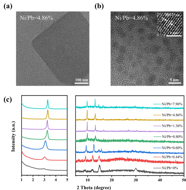
Fig. 2 HRTEM images of (a) the deep blue nanosheet and (b) \text{FAPbBr}_3 QDs (Ni/Pb = 4.86%). Inset: Lattice distances of QDs. (c) XRD patterns of \text{FAPbBr}_3 QDs (Ni/Pb = 0, 0.44, 0.60, 0.80, 1.36, 4.86 and 7.96%).
