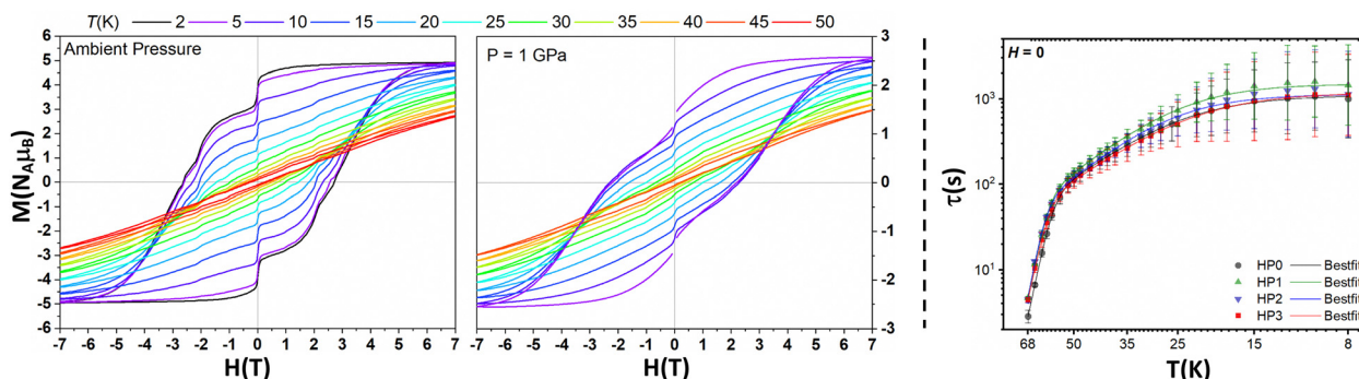
Fig. 2 Hysteresis loops of 1 at 2 K and 5–50 K in 5 K steps recorded at ambient pressure (left) and at 1 GPa (centre). For the series at 1 GPa, data below +/-800 Oe at 5 K are omitted due to the superconductive manometer (Pb). Right: Relaxation profile ( \tau vs. T ) for 1 at ambient pressure (HP0), 0.37 GPa (HP1), 0.79 GPa (HP2) and 1.2 GPa (HP3) (see Fig. S41 and S42, ESI † for fitted data and variations in the distribution of \tau ( \beta ) with temperature).
