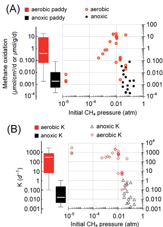
Fig. 5 Rates of aerobic methanotrophy ( n = 25 ) and anoxic methanotrophy ( n = 16 ) in rice paddy soils (A). The reaction rates and the initial methane partial pressures applied/measured during rate quantification were from the cited references in the text. (B) The fractional turnover rate.
