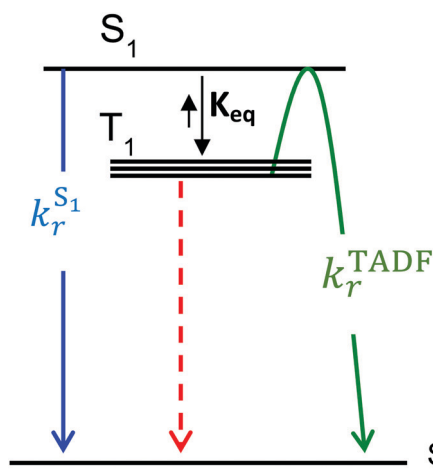
Scheme 1 The kinetic scheme for emission via TADF mechanism in two-coordinate coinage metal complex, where k_r^{S_1} and k_r^{TADF} are radiative decay rates of S_1 state and TADF process, K_{eq} indicates the equilibrium constant between S_1 and T_1 states via ISC transitions.
