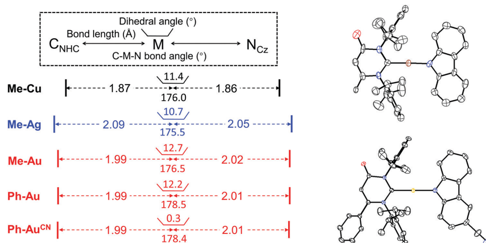
Fig. 2 Critical crystallographic data from X-ray single crystal diffraction measurements, \text{C}_{\text{NHC}} denotes the carbene carbon and \text{N}_{\text{Cz}} is the carbazolyl nitrogen. Thermal ellipsoid figures of Me-Cu (top) and Ph-Au CN (bottom).
