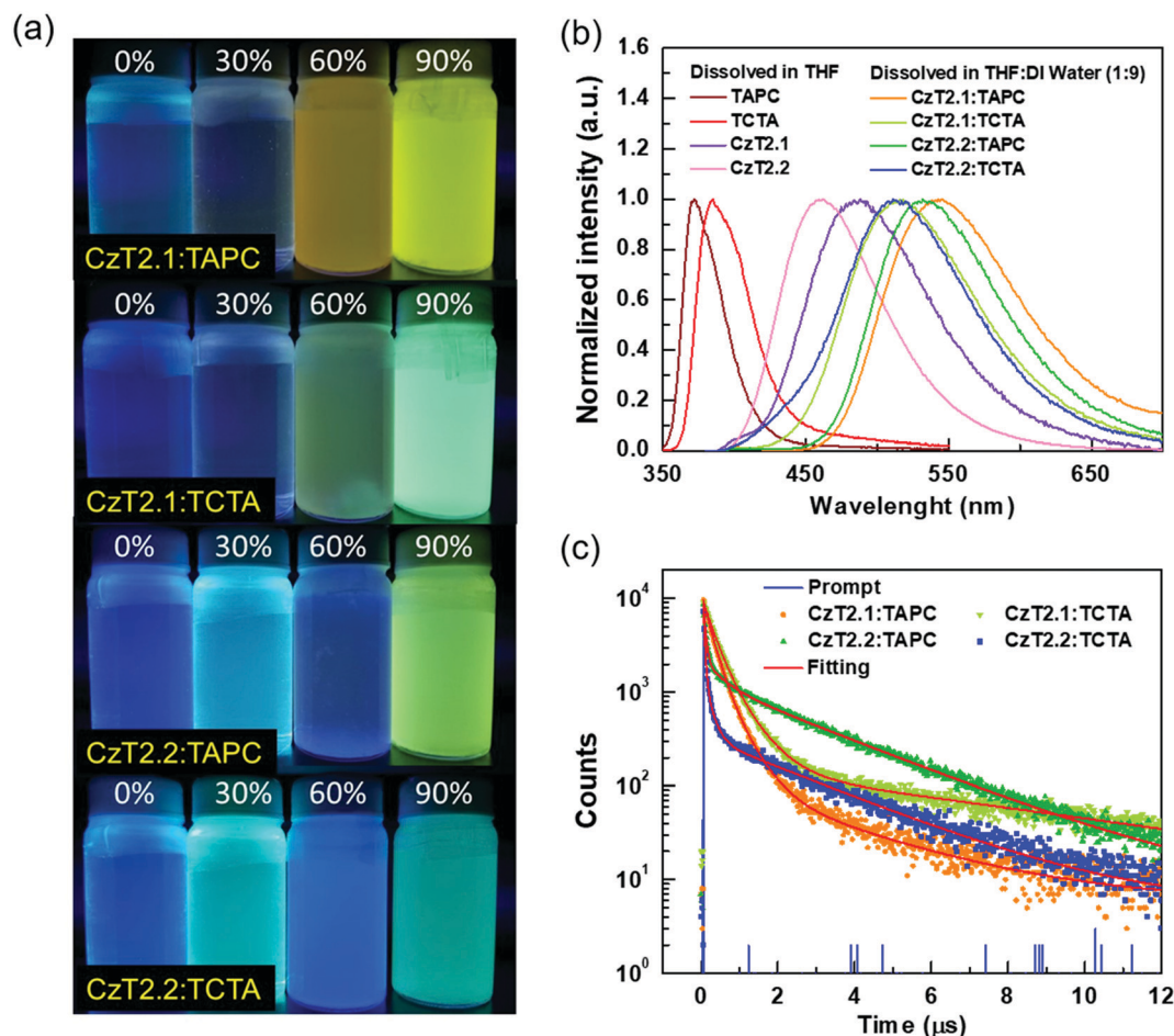
Fig. 2 (a) Photographs of four exciplex samples in THF with different water fractions under UV light illumination at room temperature, (b) normalized PL spectra of the D and A in THF and D:A (1:1) blends in THF with 90% water, and (c) the transient PL profiles of the D:A (1:1) blends in THF with 90% water.
