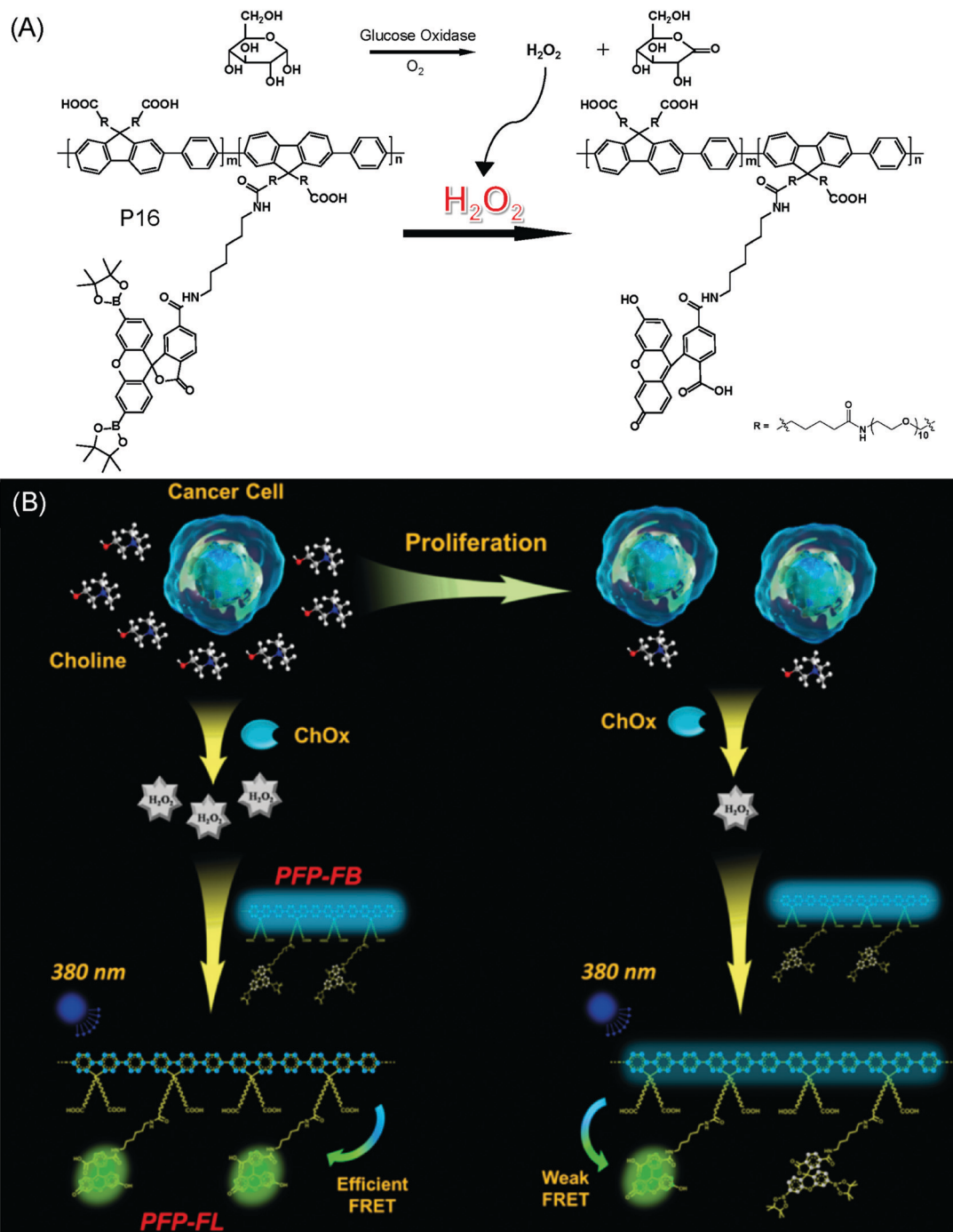
Fig. 8 Schematic illustration of H 2 O 2 -sensitive probes in the monitoring of (A) aerobic oxidation reactions and (B) the process of choline depletion in living cells. Reproduced with permission from ref. 78. Copyright 2015 American Chemical Society.
