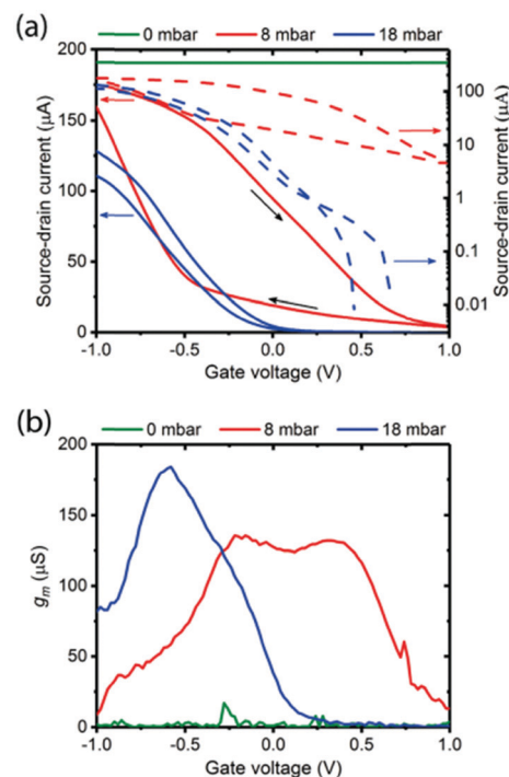
Fig. 17 (a) Hydration dependent transfer characteristics of a melanin-based OECT at 0 mbar water vapour pressure (green line), 8 mbar (red line) and 18 mbar (blue line). On/off ratio is approximately 220 at 8 mbar and approximately 10^4 at 18 mbar pressure. The corresponding transconductances ( i.e. derivative of the transfer curve). Reproduced from ref. 80 with permission from the Royal Society of Chemistry. 80
