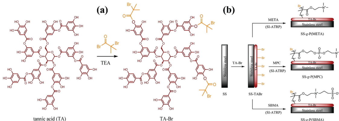
Fig. 4 (a) Synthesis of the TABr initiator primer through bromination of TA. (b) Schematic illustration of surface functionalization process with cationic and zwitterionic polymer brushes onto SS substrate via "grafting-from" approach (reprinted with permission from ref. 96. Copyright © 2015, American Chemical Society).
