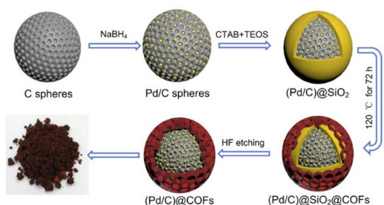
Fig. 8 Schematic synthesis procedure of (Pd/C)@TpPa (reproduced from ref. Li et al. , J. Colloid Interface Sci. , 2021, 591 , 273–280 copyright 2021 Elsevier Inc. All rights reserved).
