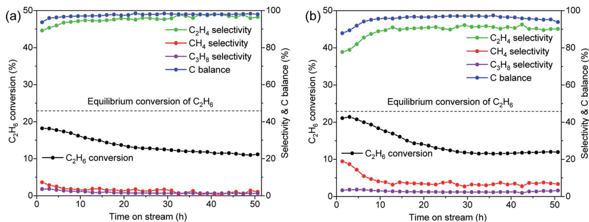
Fig. 8 Catalytic performances of (a) 0.5Co@MFI and (b) 1.3Co@MFI catalysts at 7.5 bar pressure. Reaction conditions: 50 mg catalyst, pretreatment by 10% \text{H}_2/\text{N}_2 for 30 min, 20% \text{C}_2\text{H}_6/\text{N}_2 , 5 \text{mL min}^{-1} , 650 °C.
