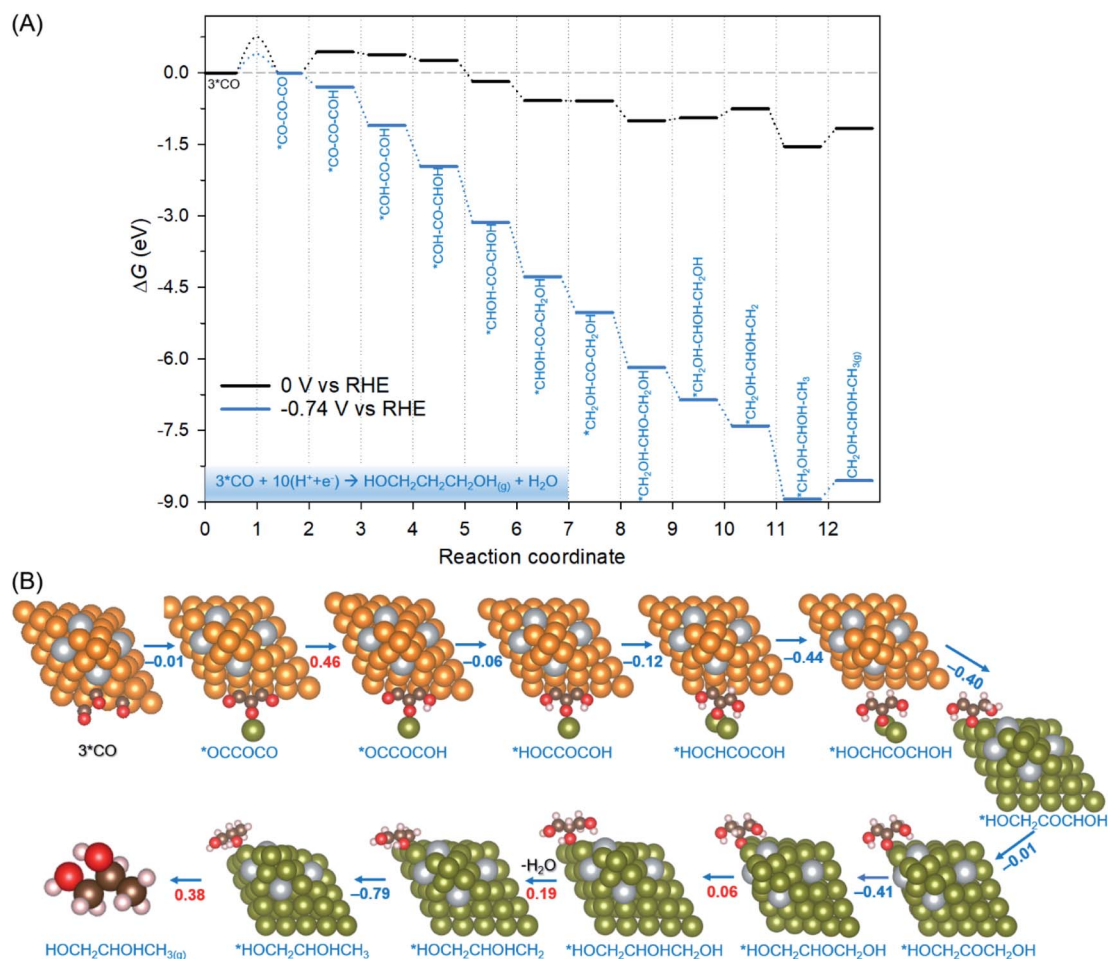
Fig. 5 Reduction of *CO to 1,2-propanediol on the Ag-doped Cu-DAN. (A) Preferred pathway and associated reaction energetics identified for the production of 1,2-propanediol starting with 3*CO on the Ag-doped Cu-DAN surface at 0 V and -0.74 V (corresponding to the 0.40 eV barrier threshold) vs. RHE (B) atomic structures of the reaction intermediates along the pathway. In the upper panel, one or two Cu atoms bonded with O denote the adjacent nanopillars (in green), after the formation of *CHOH-CO-CHOH, intermediates have completely adsorbed on the adjacent nanopillars. Free energy change ( \Delta G ) values are in eV. Blue and red values denote the exergonic and endergonic processes, respectively. Colour code: Cu, orange and green; C, brown; O, red; H, pink.
