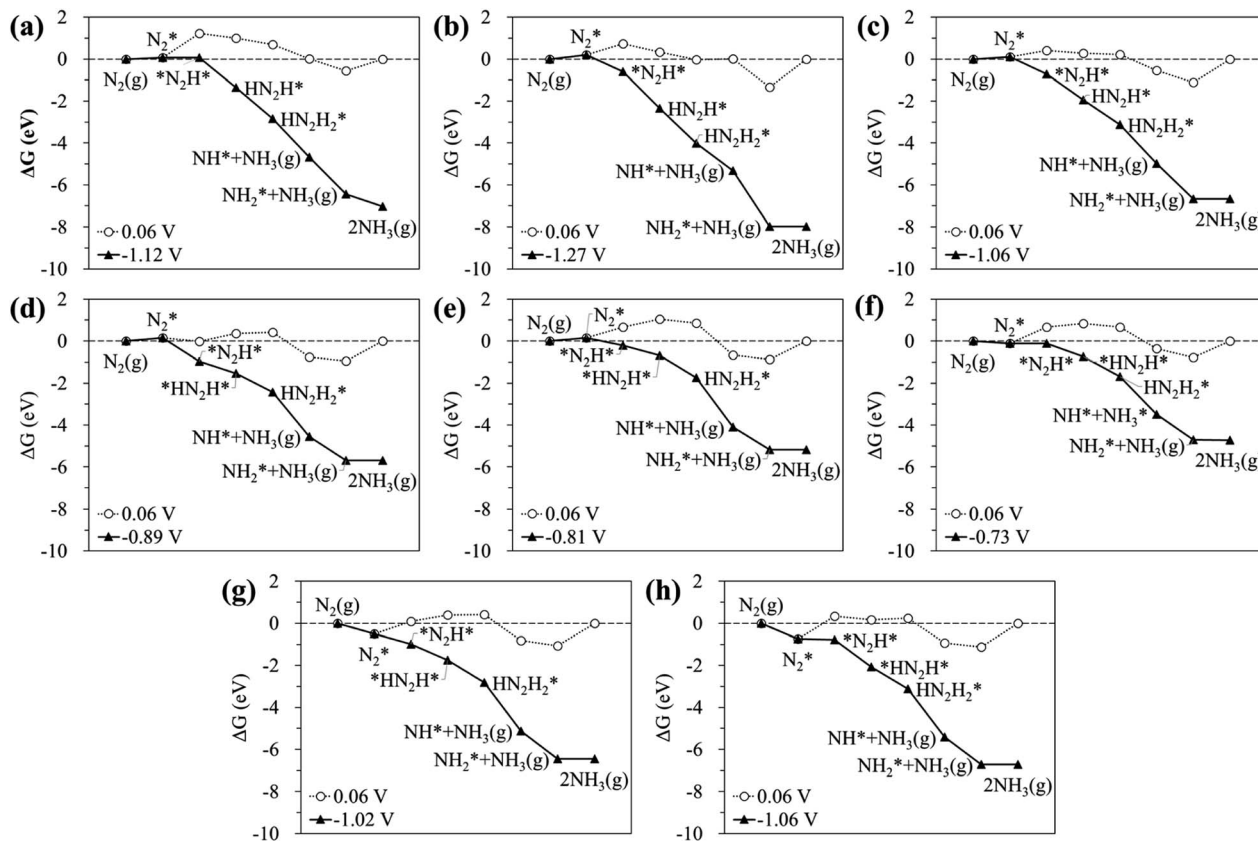
Fig. 6 Calculated Gibbs free energy profiles at equilibrium (O) and limiting (▲) potentials for the N_2 RR on hetero-RuM DACs of group I [(a) RuTi/C, (b) RuV/C, and (c) RuCr/V], group II [(d) RuSc/C, (e) RuMn/C, and (f) RuFe/C], and group III [(g) RuCo/C and (h) RuNi/C] via the most favourable pathway.
