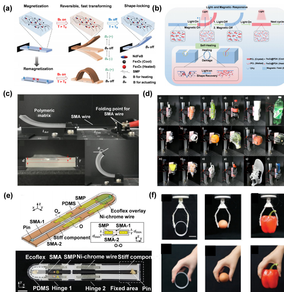
Fig. 8 (a) Working machine of magnetic SMP. 250 Copyright 2019, WILEY-VCH. (b) Schematic diagram of light- and magnetic-responsive actuation and shape memory assisted self-healing. 251 Copyright 2021, The Royal Society of Chemistry. (c) SMA actuator and the bending deformation. (d) Schematic diagram of SMA grasping various objects. 252 Copyright 2019, Springer Nature. (e) Schematic diagram of the soft finger assembly structure and its top view of the structure. (f) Schematic diagram of the prepared soft gripper imitating a human hand gripping objects (low to high stiffness). 257 Copyright 2017, Mary Ann Liebert, Inc.
