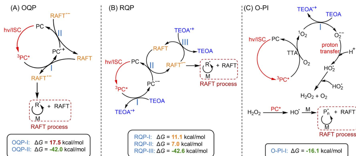
Scheme 2 Proposed mechanism of photo-RAFT polymerization catalyzed by \text{ZnPcS}_4^- via three pathways. a Note: (A) PET-RAFT polymerization via an oxidative quenching pathway (OQP) and (B) a reductive quenching pathway (RQP). (C) Photo-RAFT polymerization via an oxygen-mediated photoinitiation (O-PI) system. Values indicate the Gibbs free energy change (ΔG) of electron transfer reactions in three pathways calculated by DFT (coordinates and energies of PC, RAFT agent, TEOA, and \text{O}_2 were shown in ESI†).
