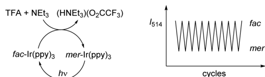
Fig. 2 Acid-base treatment followed by irradiation allows repetitive cycling between fac - and mer - \text{Ir(ppy)}_3 . The interference of accumulating (\text{HNET}_3)(\text{O}_2\text{CCF}_3) is low for the first ten cycles, as evidenced by spectroscopic monitoring.
