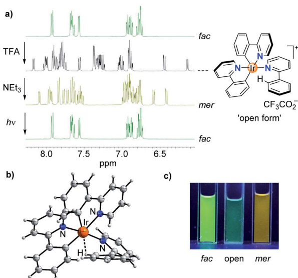
Fig. 1 (a) ^1\text{H} NMR spectra (400 MHz, \text{CD}_2\text{Cl}_2 , aromatic region) for the conversion of \text{fac-Ir(ppy)}_3 into \text{mer-Ir(ppy)}_3 and back. (b) Molecular structure of [\text{Ir(ppy)}_2(\text{Hppy})](\text{NTf}_2) in the crystal with thermal ellipsoids at 50% probability; the anion is not shown for clarity. (c) Photos of solutions containing \text{fac-Ir(ppy)}_3 , [\text{Ir(ppy)}_2(\text{Hppy})](\text{O}_2\text{CCF}_3) ('open form'), and \text{mer-Ir(ppy)}_3 under UV-light ( \lambda_{\text{ex}} = 366 \text{ nm} ).
