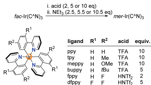
Scheme 2 Chemically induced fac \rightarrow mer isomerizations are possible for different \text{Ir(C}^{\wedge}\text{N)}_3 complexes using either TFA or \text{HNTf}_2 for the protonation step.
