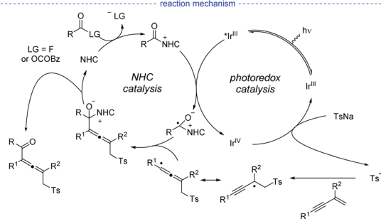
Scheme 19 NHC/Ir co-catalyzed three-component 1,4-sulfonylacylation of 1,3-enynes.
