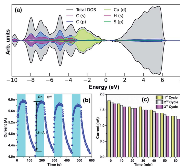
Fig. 8 (a) PDOS analysis of \text{Cu}_{18} NC. (b) Photoresponse properties of the \text{Cu}_{18} NC and (c) their reproducibility.
