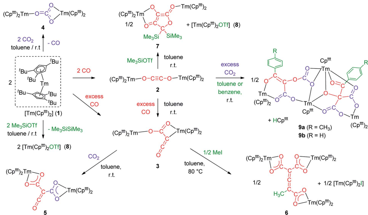
Scheme 5 Summary scheme of all the reactivity described in this study starting from [Tm(Cp^{ttt})_2] (1).
