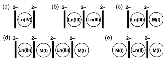
Scheme 1 Depiction of crystallographically characterized homoleptic Ln complexes with the \text{COT}^{2-} ligand.
