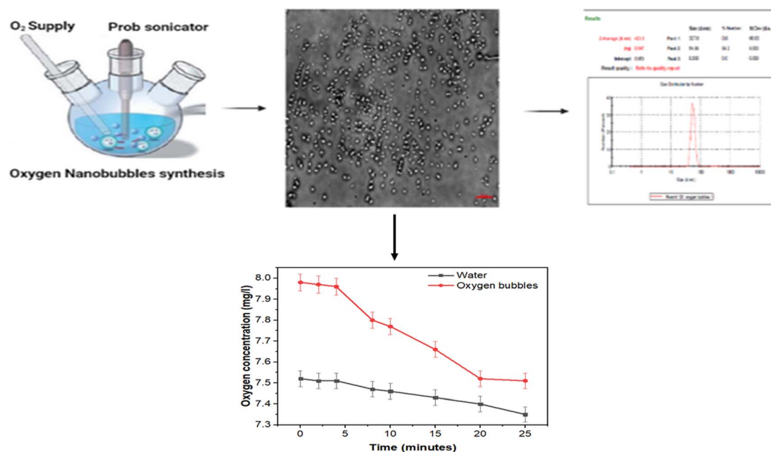
Fig. 8 Fabrication and characterization of ONBs.
