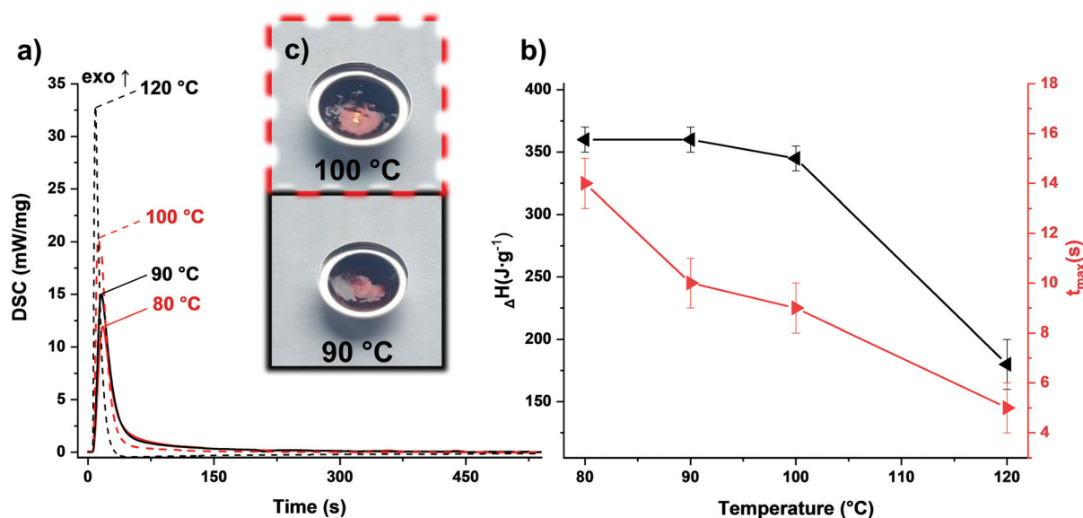
Fig. 5 (a) Photo-DSC of the TOMDA-formulation at 80–120 °C, 2 \times 900 s, 320–500 nm, 60 \text{ mW cm}^{-2} . (b) Temperature dependence of photo-DSC results for the TOMDA-formulation: enthalpy change ( \Delta H black) and time until maximal heat is released ( t_{\max} red). (c) Cured Samples at 90 & 100 °C.
