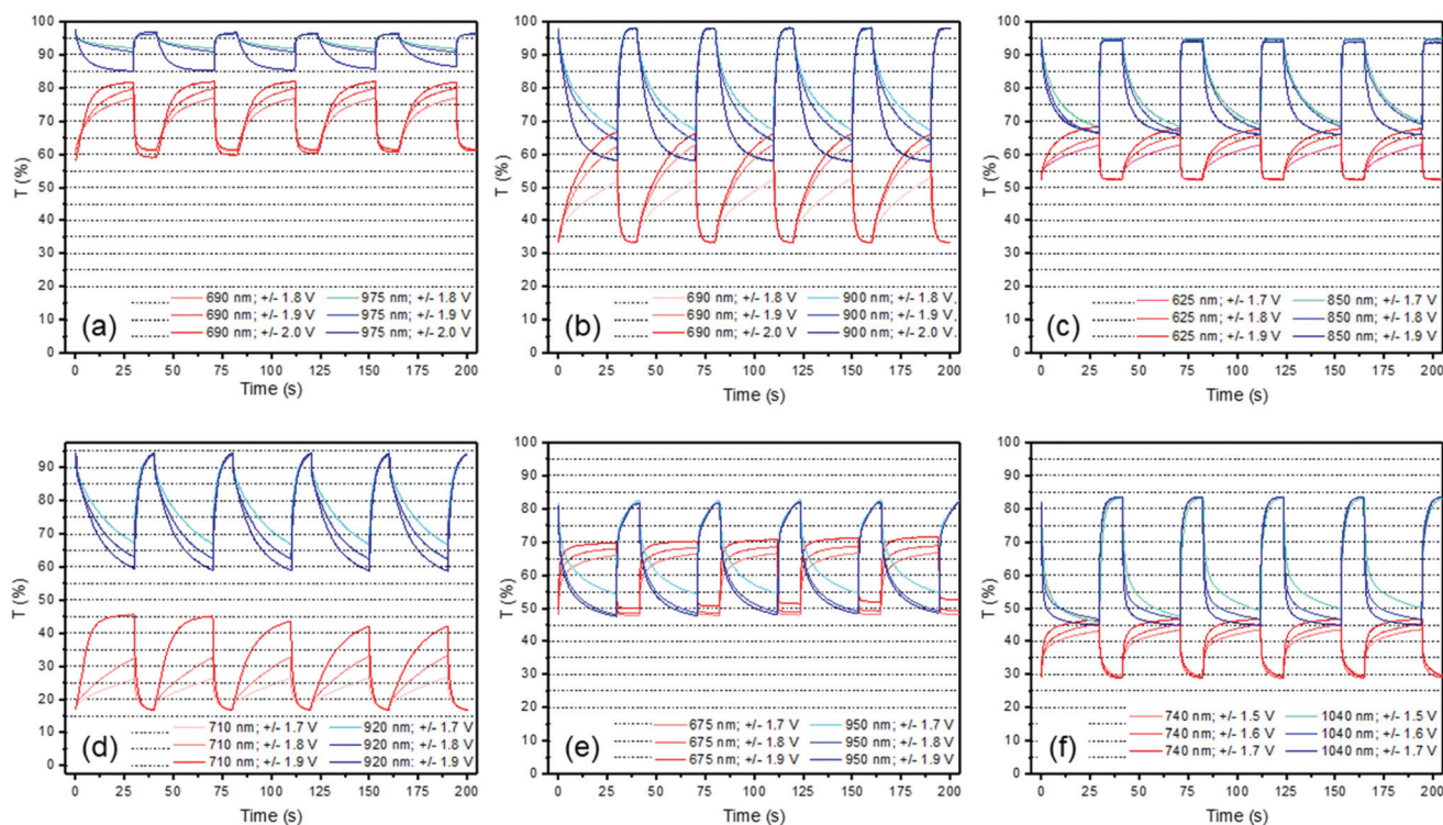
Fig. 3 Square-wave potential step absorptimetry of ECDs containing polymers (a) p(\text{IID-T}) , (b) p(\text{IID-2T}) , (c) p(\text{IID-3T}) , (d) p(\text{IID-TT}) , (e) p(\text{IID-EDOT}) and (f) p(\text{IID-2EDOT}) undergoing five cycles of EC switching at different voltages at 30 s/10 s oxidation/reduction intervals.
