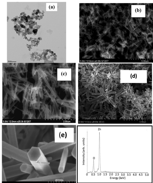
Fig. 3 (a) TEM image of ZnO nanoparticles used as a seed layer for ZnO nanorods growth on a Si substrate with scale bar of 200 nm. (b) and (c) SEM images of ZnO nanorods grown in the solution phase without a seed layer, (d) and (e) ZnO nanorods grown on the pre-coated Si substrate with ZnO nanoparticles. (f) EDS spectrum of a ZnO nanorod sample grown on a Si substrate with the ZnO seed layer.
