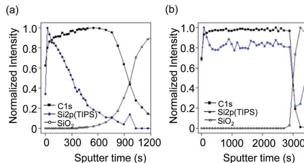
Fig. 4 XPS depth profiles of a TIPS-P/CuSP blend film coated from (a) ODCB and (b) \text{CHCl}_3 solutions on a Si substrate.
