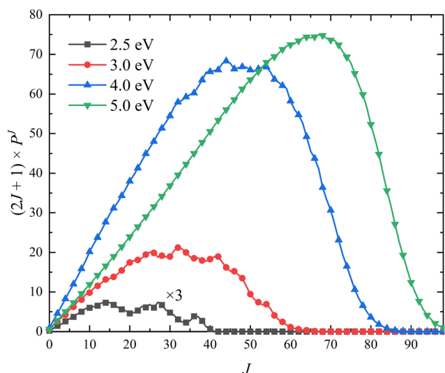
Fig. 7 Opacity functions of the \text{Ca}^+(\text{}^2\text{S}) + \text{H}_2(\nu_0 = 0, j_0 = 0) \rightarrow \text{CaH}^+ + \text{H} reaction at four collision energies ( E_c = 2.5, 3.0, 4.0 and 5.0 eV) calculated by the TDWP method on the PIP-NN PES.
