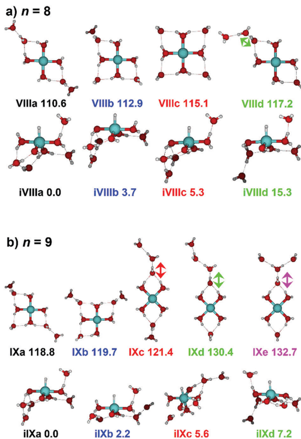
Fig. 5 Calculated intact and inserted isomers of (a) V^+(H_2O)_8 and (b) V^+(H_2O)_9 . All isomers were calculated at the B3LYP/aug-cc-pVDZ level of theory with relative energies given in \text{kJ mol}^{-1} inclusive of zero-point energy. Arrows indicate the O–H stretch of the most red-shifted band, in each case a water molecule in a double acceptor binding motif in the second solvation sphere.
