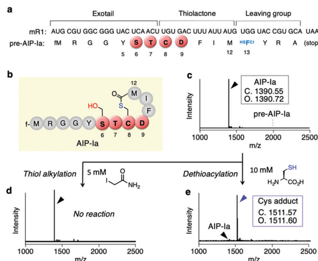
Fig. 2 One-pot in vitro ribosomal synthesis of the AIP-I analog (AIP-Ia). (a) mRNA (mR1) and precursor peptide sequence (pre-AIP-Ia) used for in vitro CTP/CDP synthesis. 3'-Acylated tRNA, ^{\text{H}^{\text{S}}\text{F}^{\text{Cl}}13} -tRNA EnAsn#3 CCA , was in vitro -prepared using a flexizyme in advance, and then used for translation in the Trp-deficient FIT system to generate a backbone thioester. f, formyl group. (b) Peptide sequence of AIP-Ia as a product. (c) MALDI-TOF MS spectrum of a crude translation product after 30 min translation. (d) Alkylation of the translation product by IAA. (e) Dethioacylation of thiolactone by addition of cysteine.
