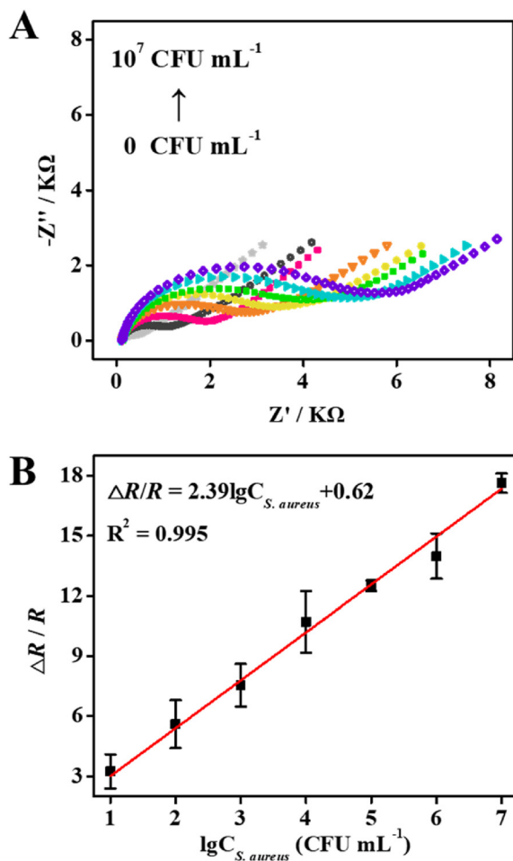
Fig. 5 (A) EIS of the BIF-based sensor for the detection of S. aureus at a series of gradient concentrations from 0 to 10^7 CFU mL -1 . (B) Corresponding calibration curve of the EIS response versus the logarithm of S. aureus concentration.
