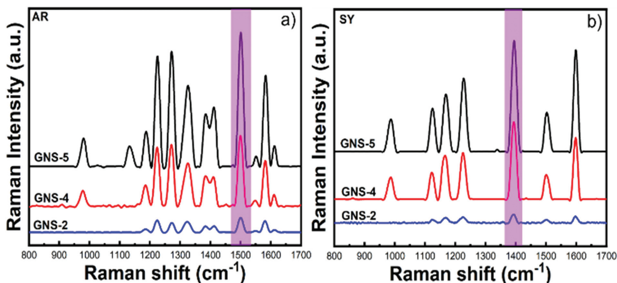
Fig. 2 Comparison of SERS signal intensity of allura red dye using GNS-2, GNS-4, and GNS-5 (a). Comparison of SERS signal intensity of sunset yellow with GNS-2, GNS-4, and GNS-5 (b).
