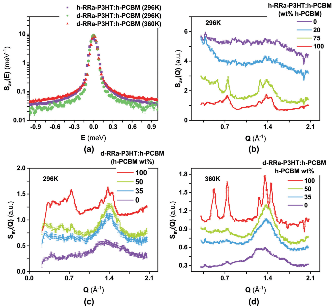
Fig. 4 (a) Q-Averaged QENS spectra at the miscibility limit. (b) Concentration-dependent neutron diffraction patterns of h-RRa-P3HT:h-PCBM at 296 K. (c) and (d) concentration-dependent neutron diffraction patterns of d-RRa-P3HT:h-PCBM at 296 K and 360 K, respectively.
