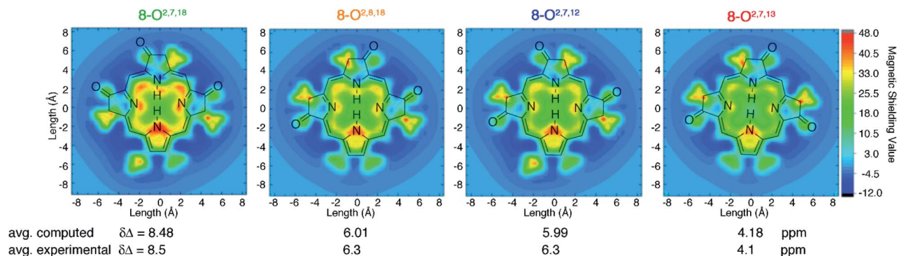
Fig. 4 Visualization of differential diatropicity in the trioxopyrrocorphin isomers: (top) isochemical magnetic shielding heat maps at a height of 1.0 Å above the macrocyclic plane and (bottom) average inner versus outer 1 H NMR chemical shifts ( \Delta\delta ). All computed quantities were obtained at the BH and HLYP/def2-TZVP level of theory. The iso-chemical shielding surface approach (ICSS) 20 a three-dimensional generalization of the nucleus independent chemical shift (NICS) technique, 21 as implemented in MultiWFN 22 was employed to visualize the spatial distribution of the ZZ component of the magnetic shielding tensor 1.0 Å above the macrocyclic plane. Note that the ethyl substituents exhibit significant diatropicity because the viewing plane bisects these groups. For further details, see ESI.†
