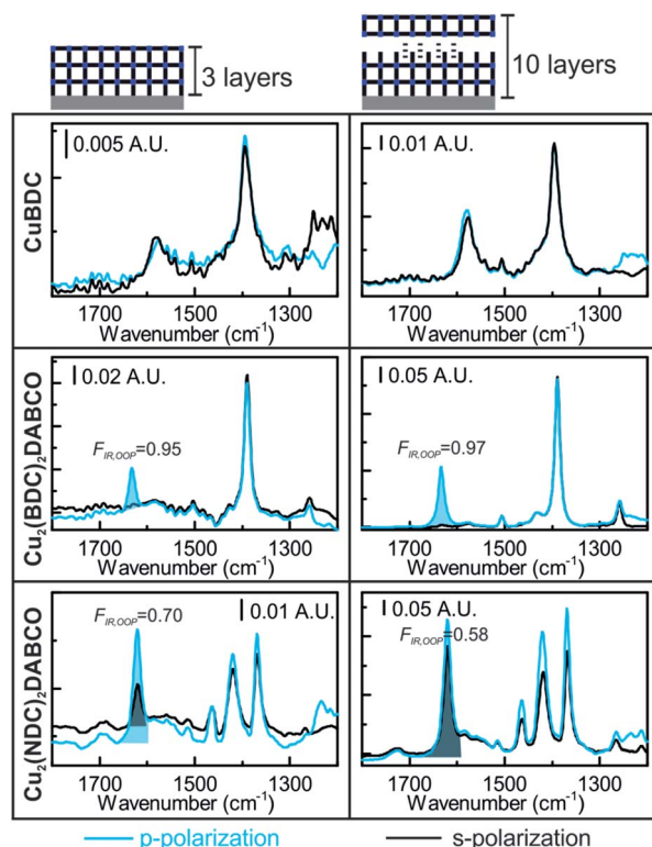
Fig. 6 Polarization-dependent ATR-IR spectra of MOF films prepared with the layer-by-layer method with 3 and 10 layers. The \nu_{\text{asym}}(\text{COO}^-) band of both 3D MOFs, Cu 2 (BDC) 2 DABCO and Cu 2 (1,4-NDC) 2 DABCO, shows strong polarization dependence, which allows to calculate the degree of out-of-plane orientation from the band areas. Background = blank Si ATR crystal.
