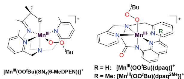
Fig. 1 Schematic structures of [Mn III (OO t Bu)(SN 4 (6-MeDPEN))] ++ (left) and [Mn III (OO t Bu)(dpaq R )] ++ (right). The [Mn III (OO t Bu)(SN 4 (6-MeDPEN))] ++ complex is a representative example of a Mn III –alkylperoxo adduct supported by an N 4 S − ligand.
